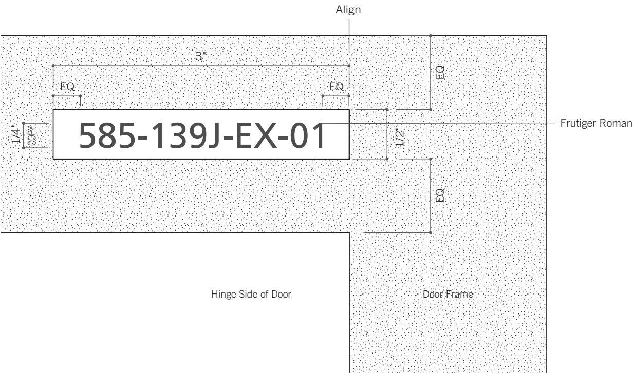
4 DETAIL - Plaque Location on Door Frame
