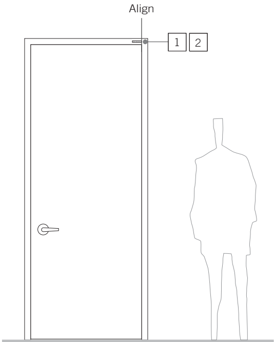
1 Door Plaque - Single Door Application
